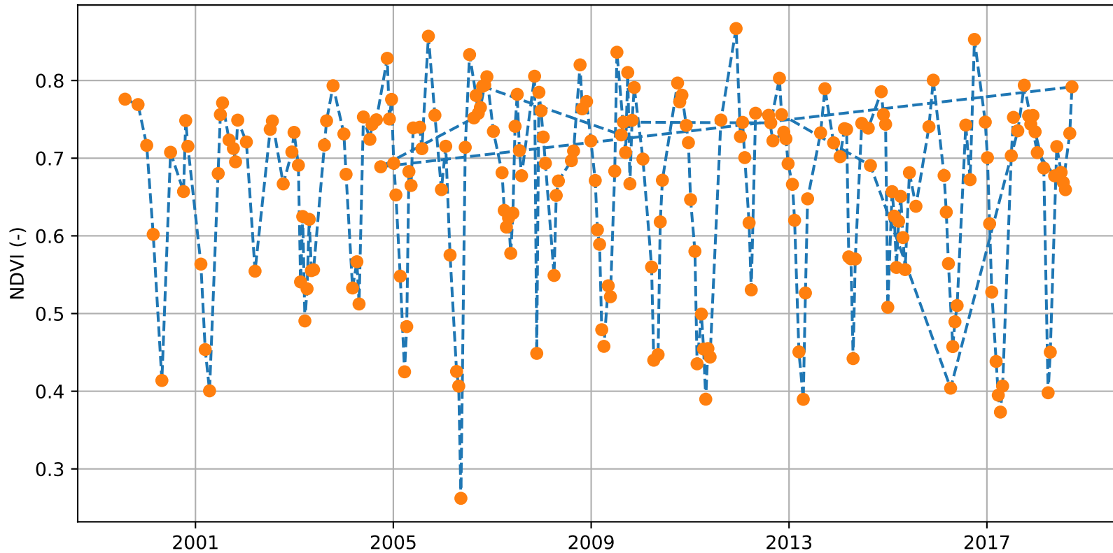
Landsat 7 NDVI time-series Uxmal
